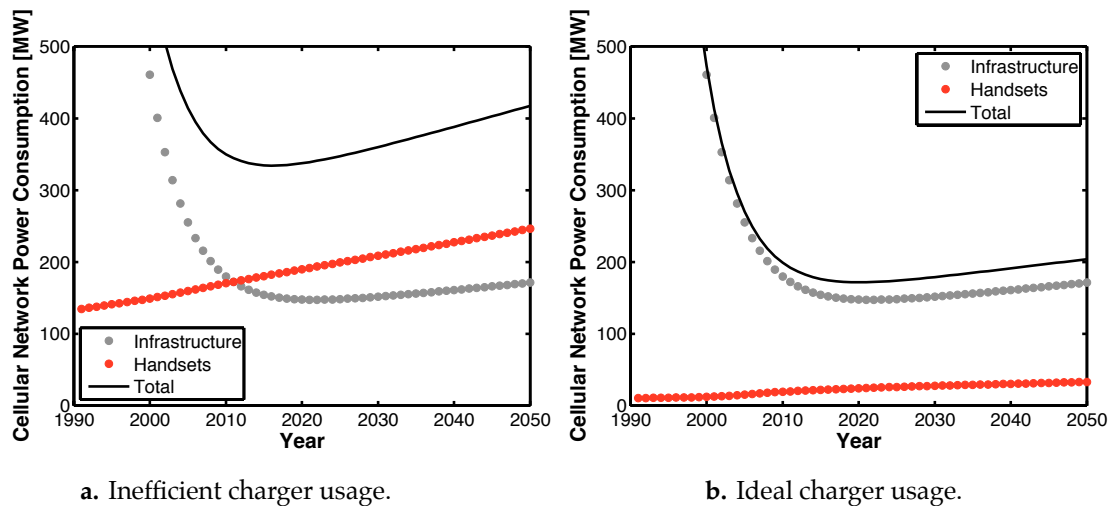
Figure 19. Predictions for the energy usage of the U.S. cellphone network for two different charge scenarios.
