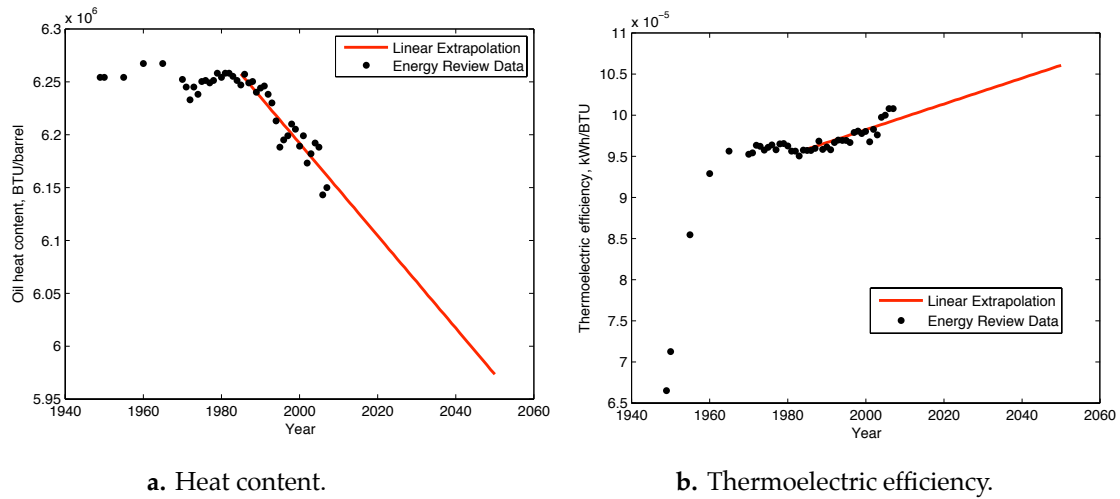
Figure 13. Heat content and thermoelectric efficiency data for oil, with extrapolations.
