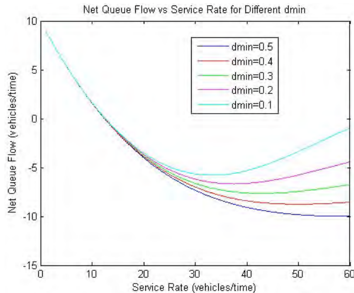
Figure 5. The relationship between r_1 and dC/dt for the congestion model with C = C_{limit} , with parameter values d_{1,max} = d_{2,max} = d_{3,max} = d_{4,max} = 2 , and C_{max} = 30 . The values of r_1 range from 1 to 60 for different values of d_{1,min} .
